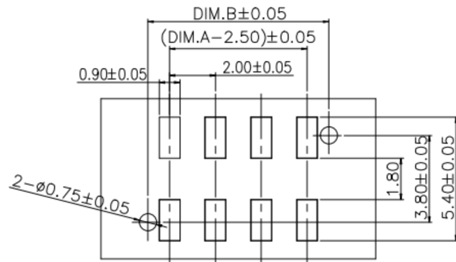
P. C. B. LAYOUT TOLERANCE: ±0.05
